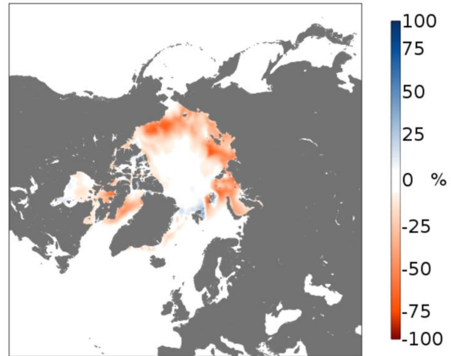
Anomaly relative to 1981-2010
